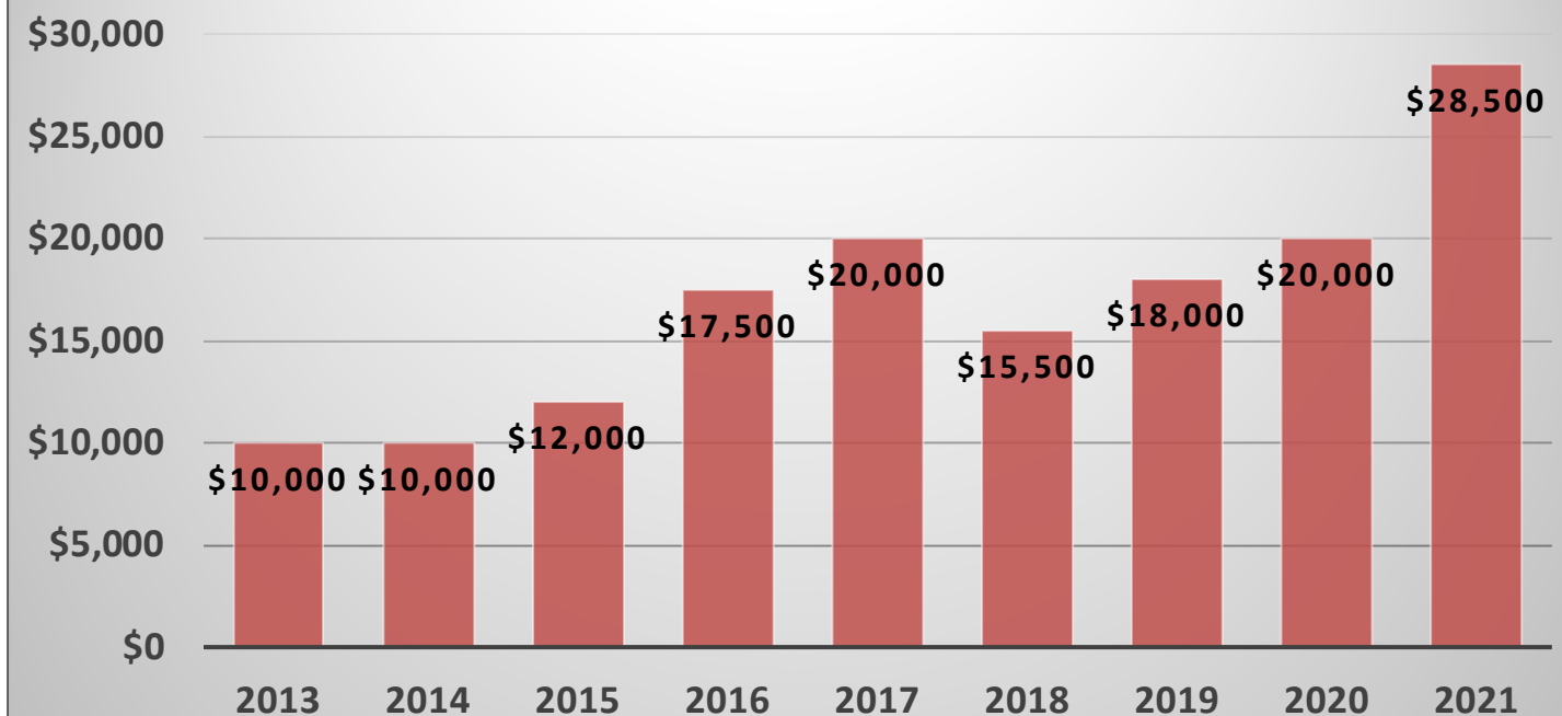
Median - Day 5
